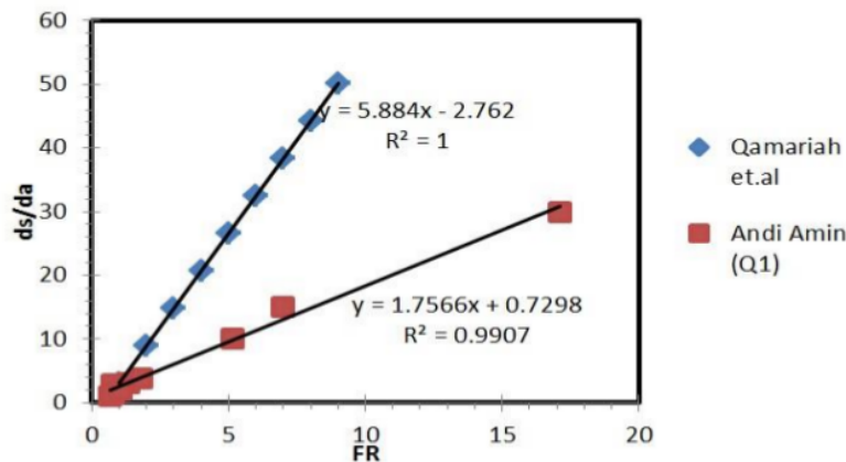
Figure 6 Relationship between froud number vs scour depth
