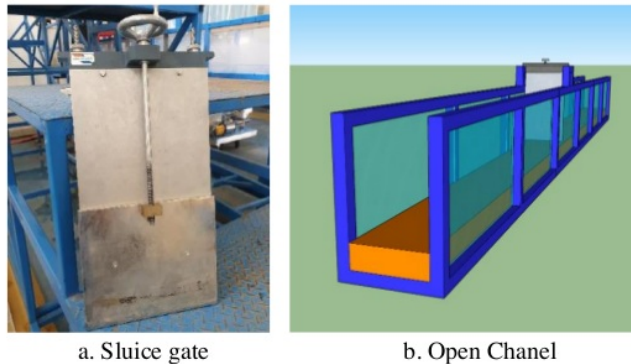
Figure 3 Physical Model of Open Channel
