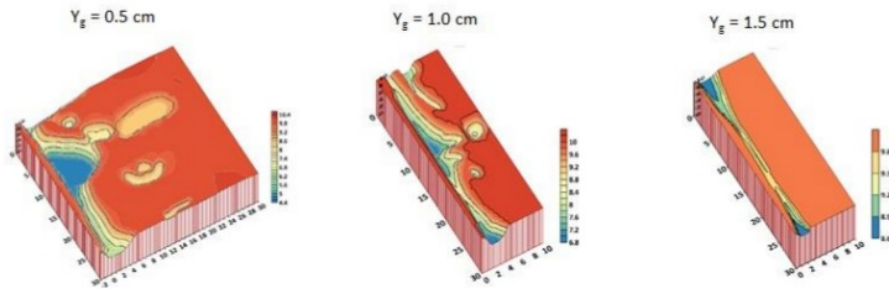
Figure 8 3 Dimensions Contour and Scour Pattern at Q = 1,406 \text{ cm}^3/\text{s} with gate openings of 0.5 cm; 1.0 cm and 1.5 cm
