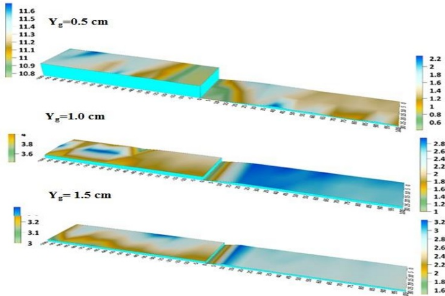
Figure 7 Flow Patterns at Q = 1,406 \text{ cm}^3/\text{s} with gate openings of 0.5 cm; 1.0 cm and 1.5 cm
