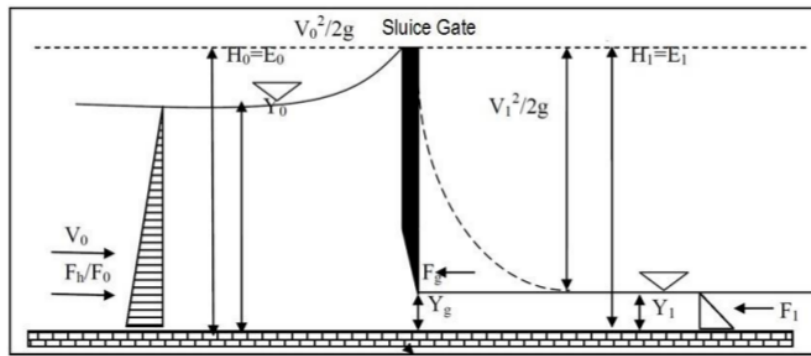
Figure 1 Flow under a sluice gate with a horizontal base
